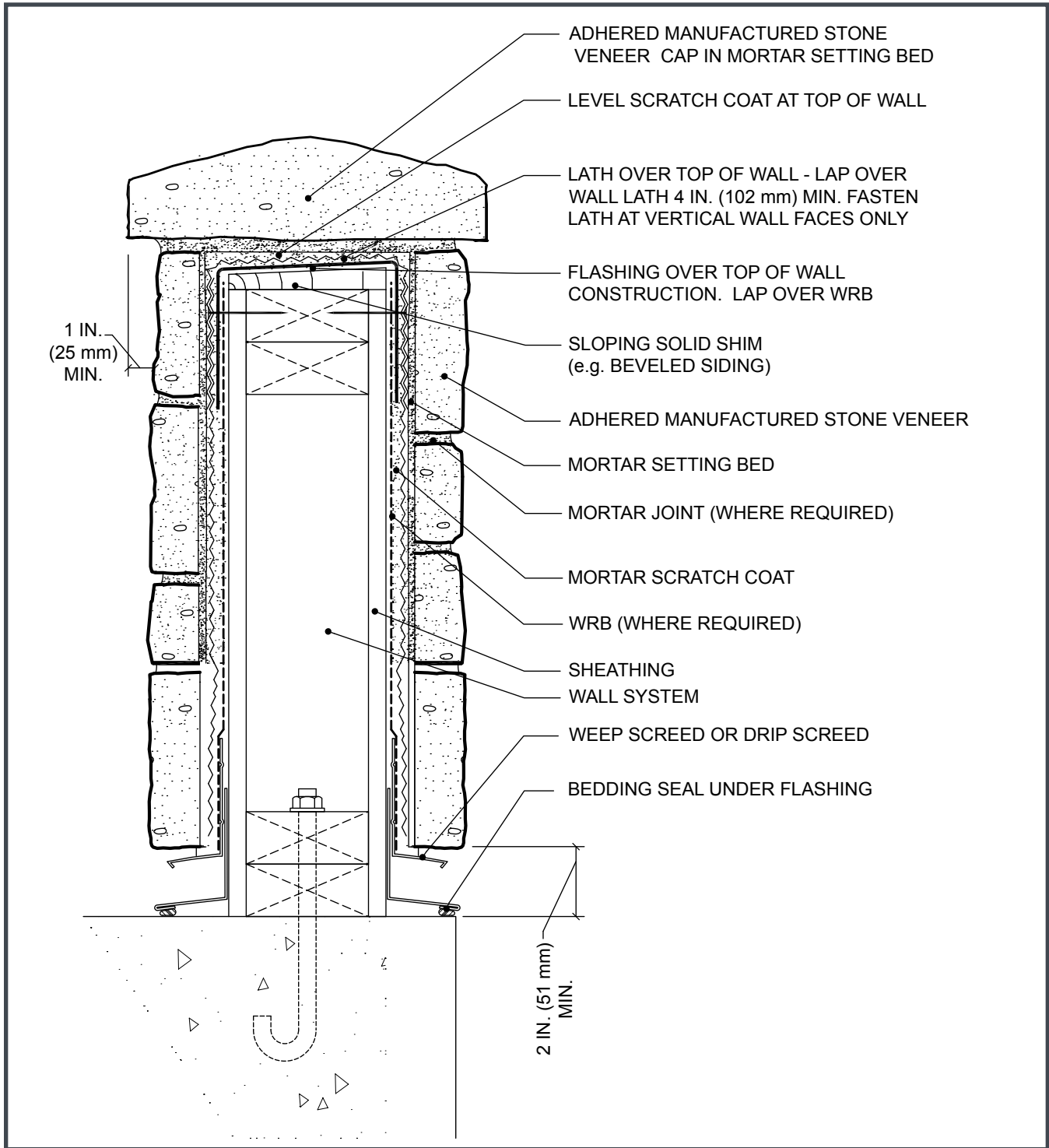
Figure 34. Wall Cap
